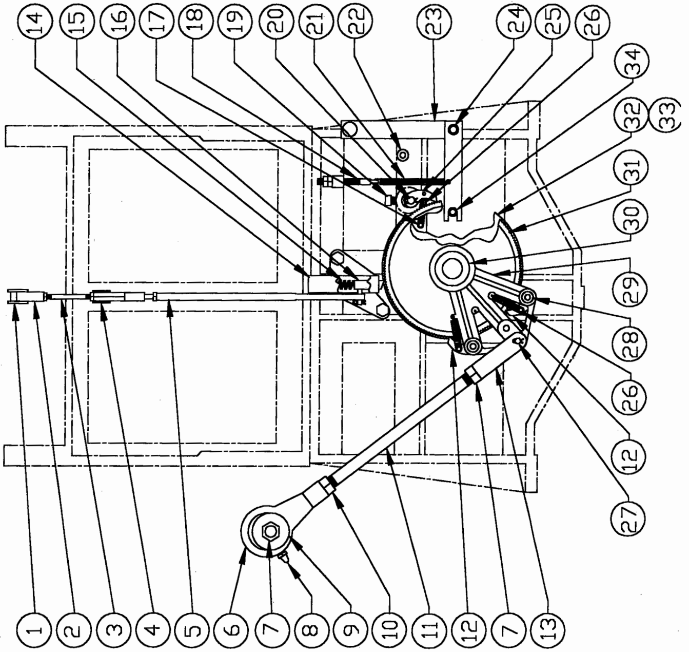
DWG. NO. NLE-A216 MODEL E5/E7/EP LABELER ABEL FEED DRIVE ASSEMBLY
