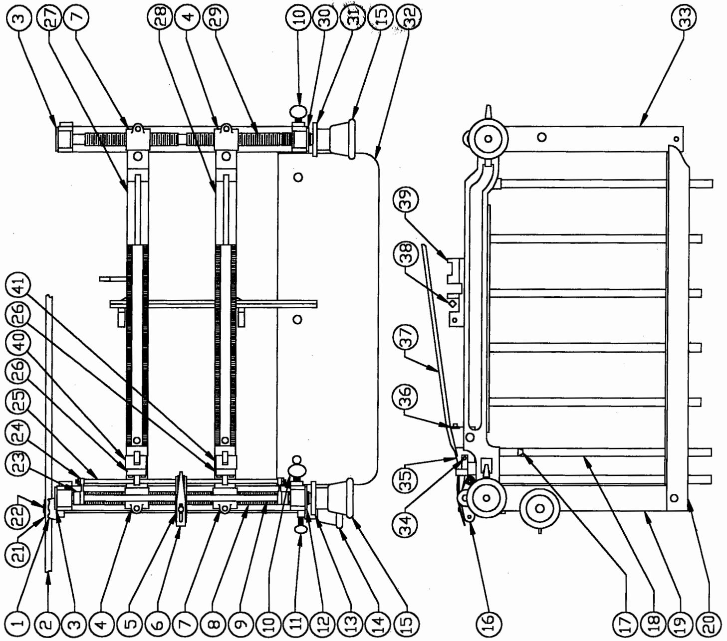
DWG. NO. NLE-A2100S MODEL E5 LABELER LABEL BED RISER & GUIDE ASSEMBLY
