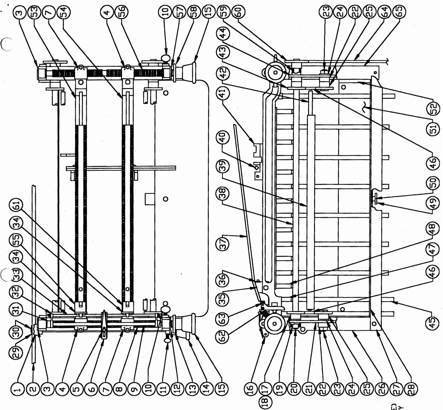
DWG. NO. NLE-A2100LCF MODEL E7/EP LABELER CONTINUOUS FEED (FLIGHT BAR TYPE) LABEL BED RISER & GUIDE ASSEMBLY
