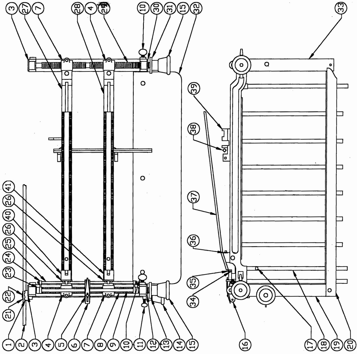
DWG. NO. NLE-A2100L MODEL E7/EP LABELER LABEL BED RISER & GUIDE ASSEMBLY
