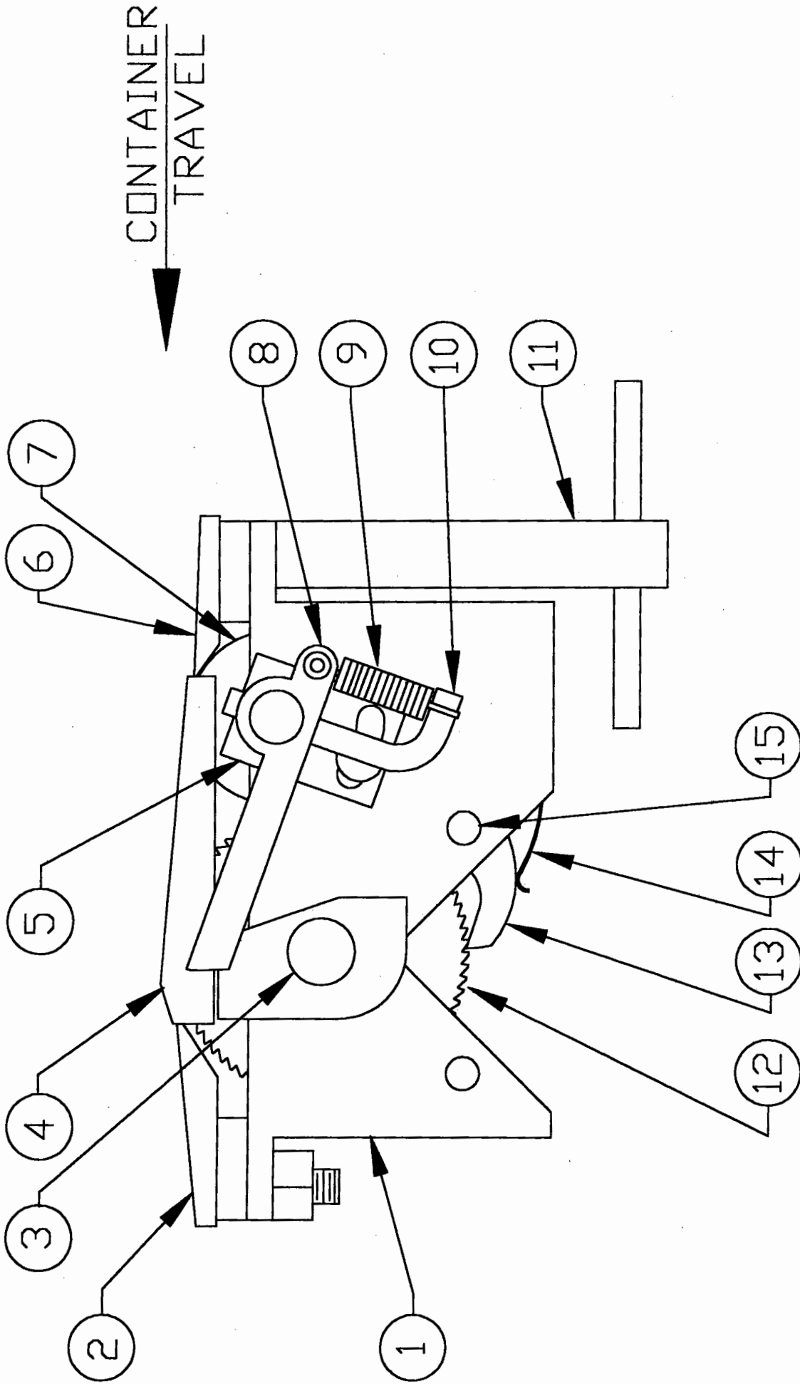
DWG. NO. NLE-A1225R MODEL AP/EP LABELER R.H. BAIL EAR TIMER ASSEMBLY WITH STOP
