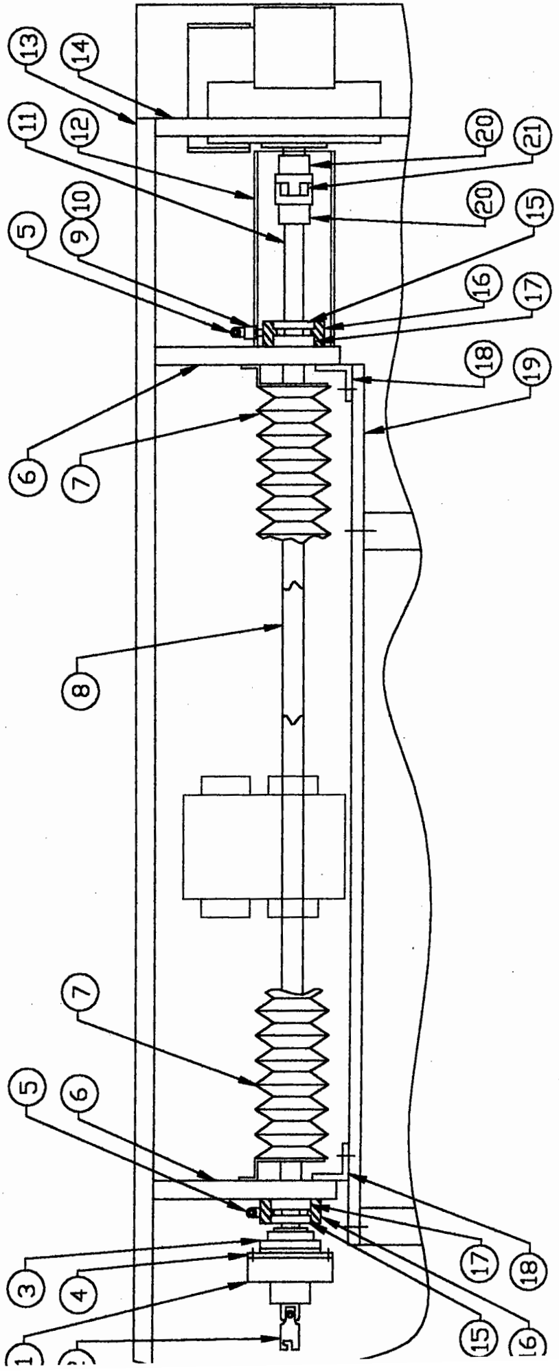
DWG. NO. NAL-A71PL MODEL A7/AP LABELER WIRE BELT PASTE DRIVE AND SUPPORT ASSEMBLY
