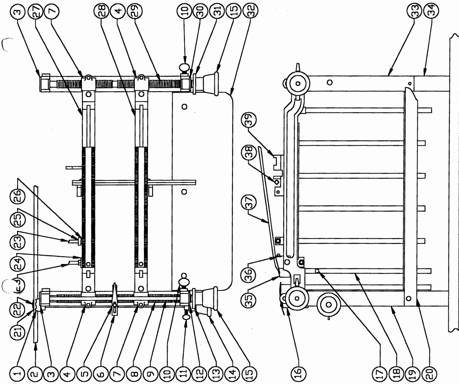
DWG. NO. NAL-A2100S MODEL A5 LABELER BEL BED RISER & GUIDE ASSEMBLY
