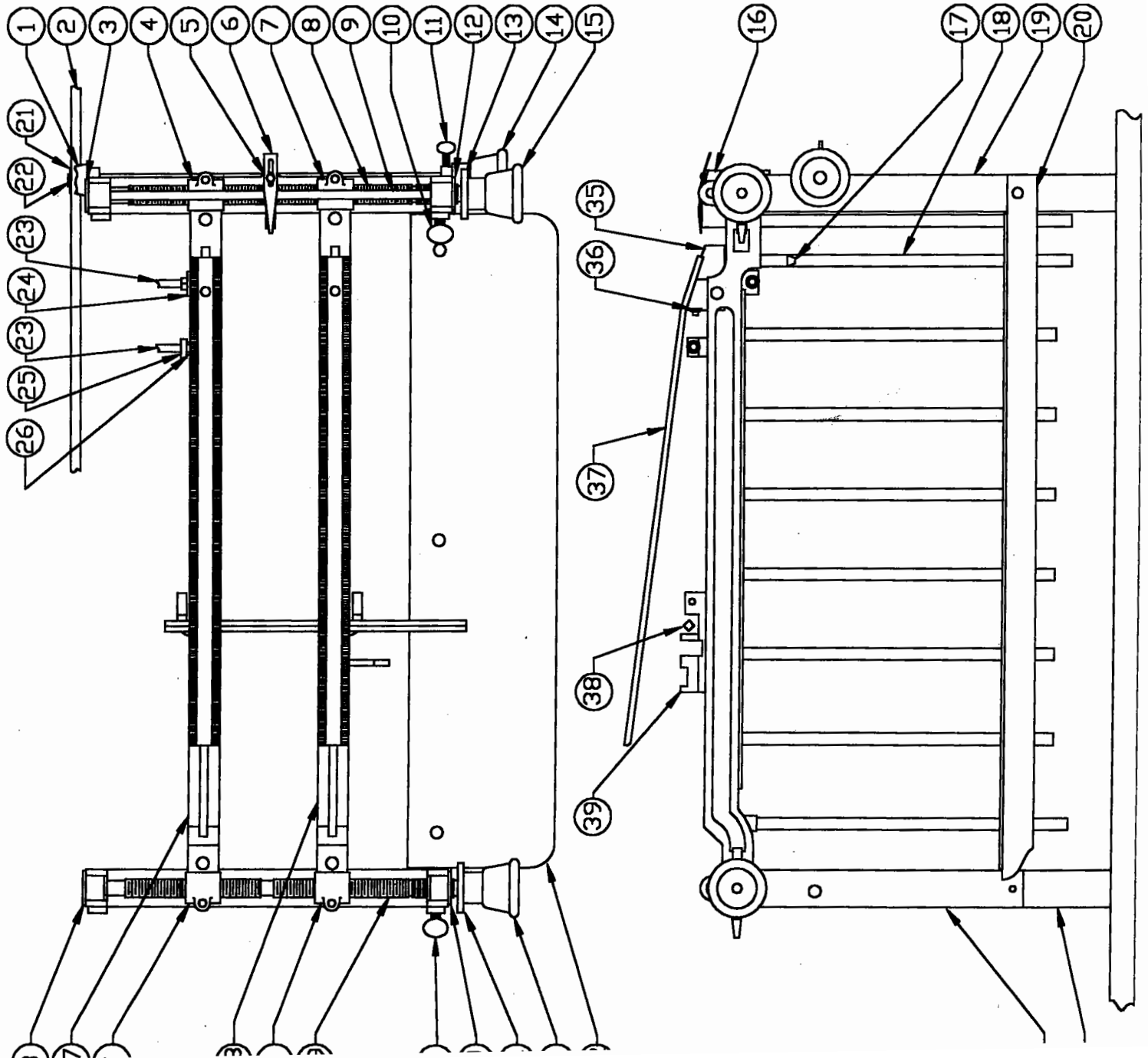
DWG. NO. NAL-A2100LRC MODEL A7RC/APRC L.H. CONTROL LABELER LABEL BED RISER & GUIDE ASSEMBLY
