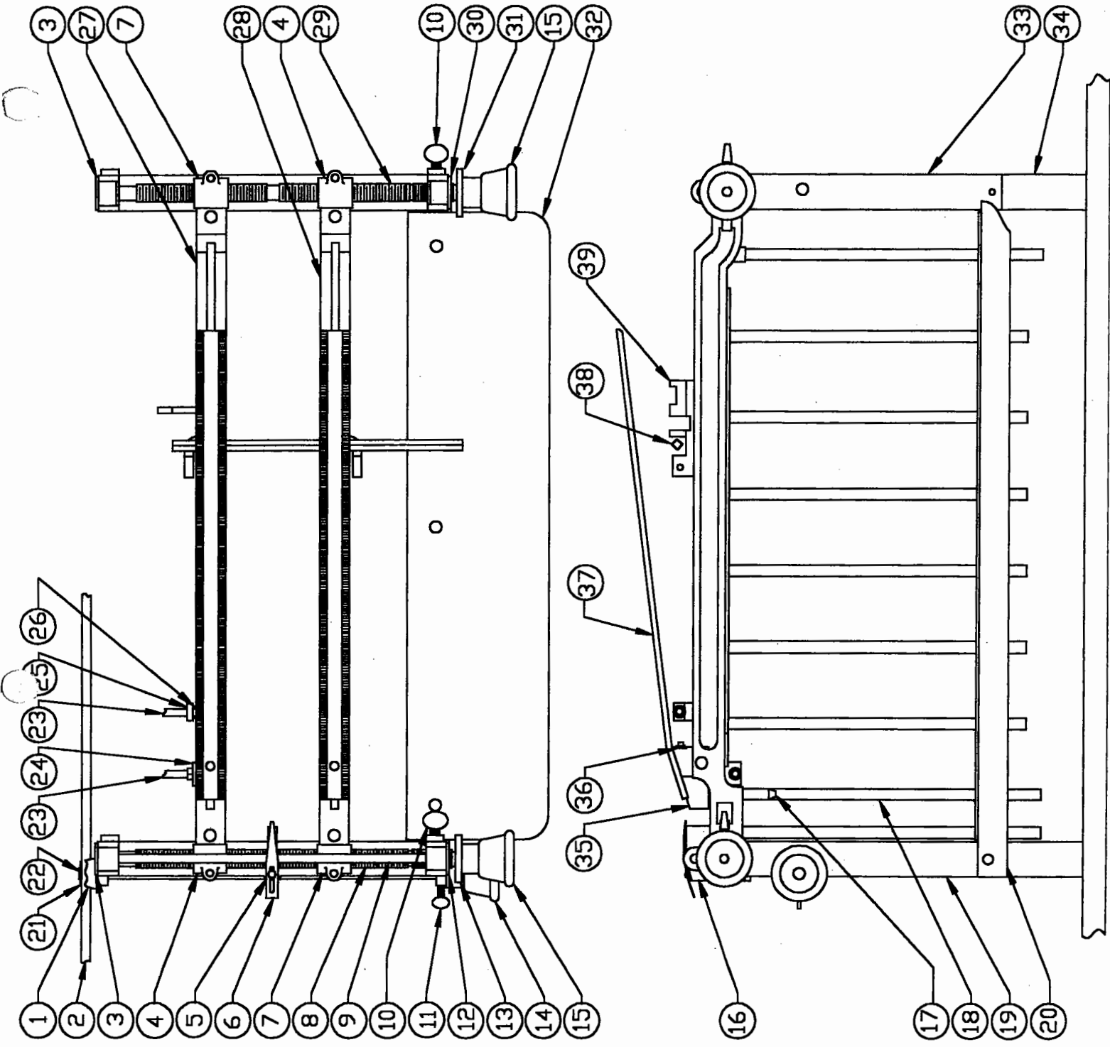
DWG. NO. NAL-A2100L MODEL A7/AP LABELER IEL BED RISER & GUIDE ASSEMBLY
