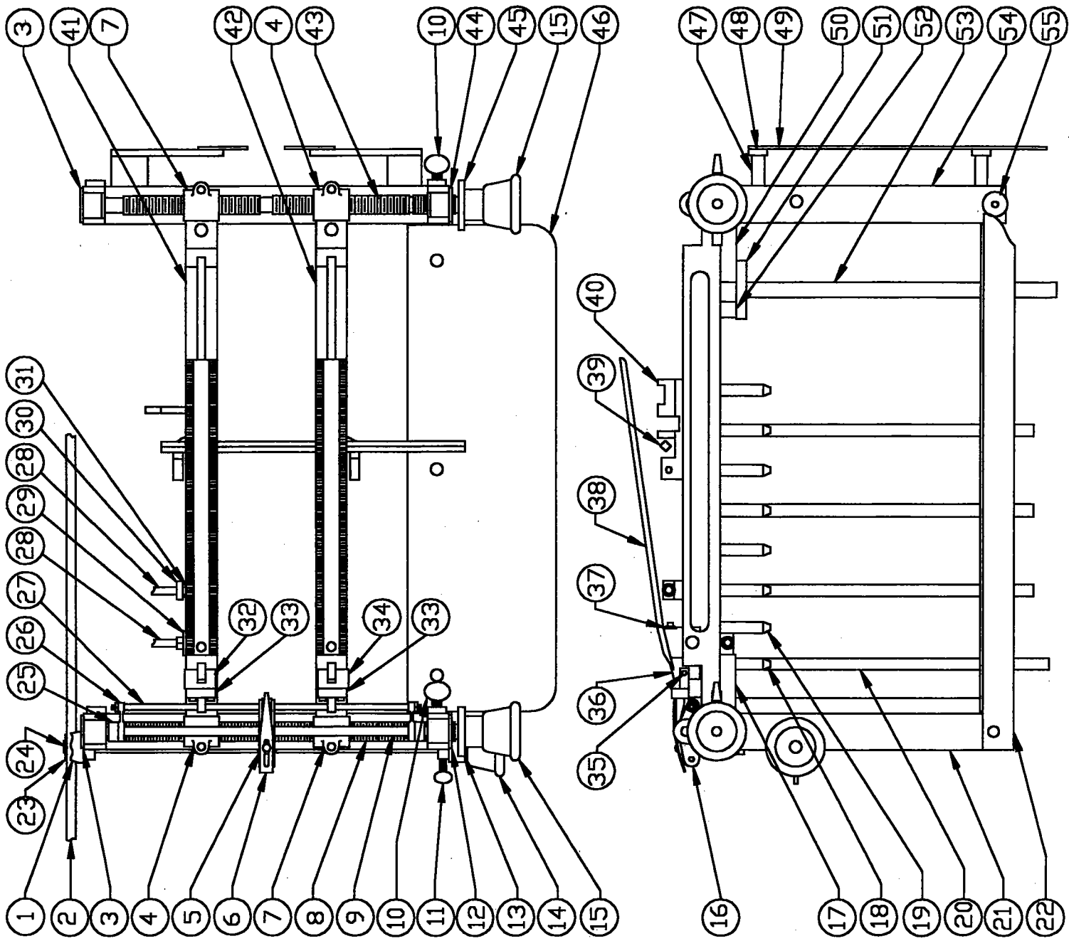
DWG. NO. NA-A2100SCT MODEL SAS LABELER CONTINUOUS FEED (TOGGLE FINGER TYPE) LABEL BED RISER & GUIDE ASSEMBLY
